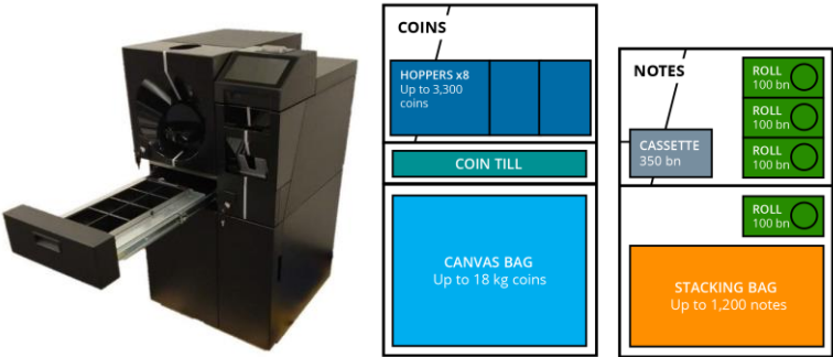
INLANE 400 DEPO PLUS STACKING
